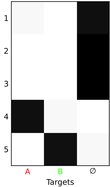
Unbalanced Sink. (high reg_pred)
