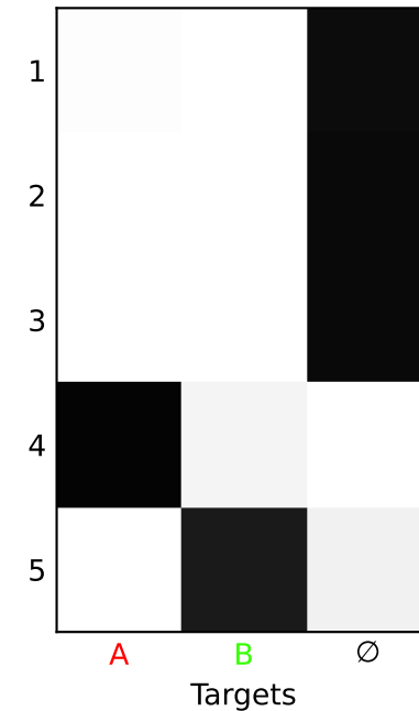
Balanced Sinkhorn
